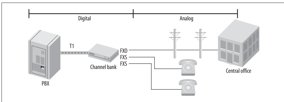
Figure 2-2. One way you might connect a channel bank
